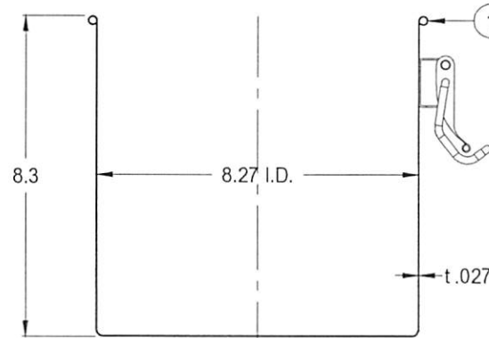
A-A SECTION VIEW
