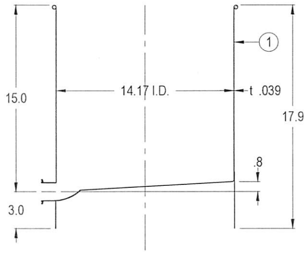
A-A SECTION VIEW
