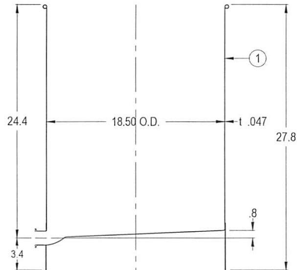
A-A SECTION VIEW
