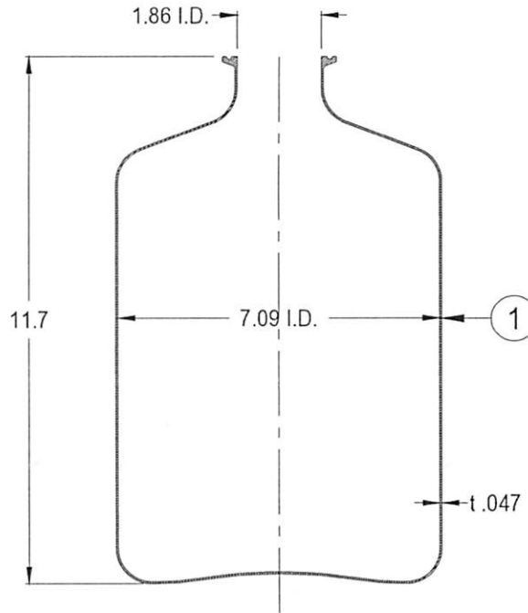
A-A SECTION VIEW
